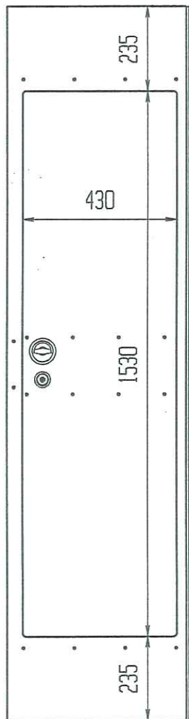
NFDH-235 17.9kg
