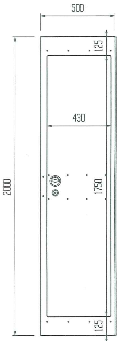
NFDH-125 17.9kg
